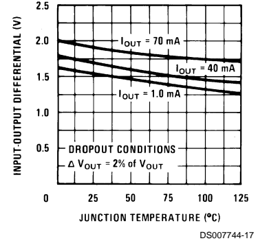
Dropout Voltage
