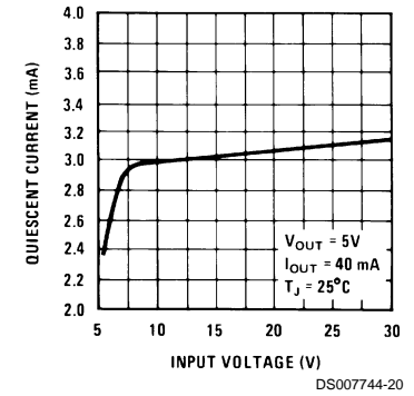
Quiescent Current
