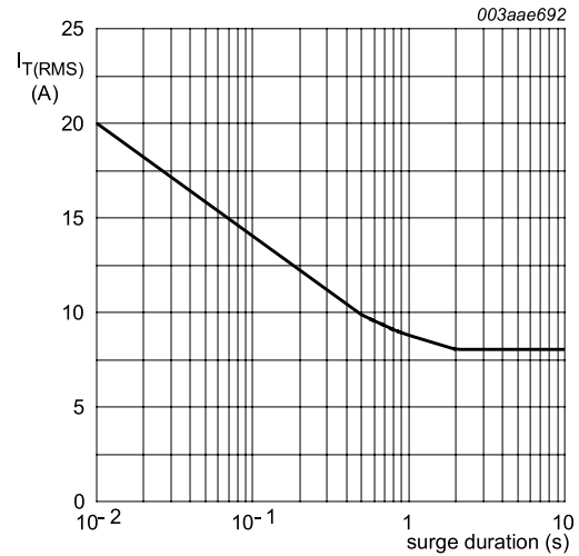
Fig. 2. RMS on-state current as a function of surge duration; maximum values f = 50 Hz; T_{mb} \leq 102\text{ }^{\circ}\text{C}
